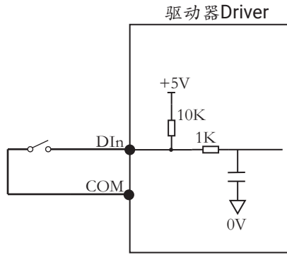
开关（继电器）接线示意图 Wire Diagram of Switch (relay)
